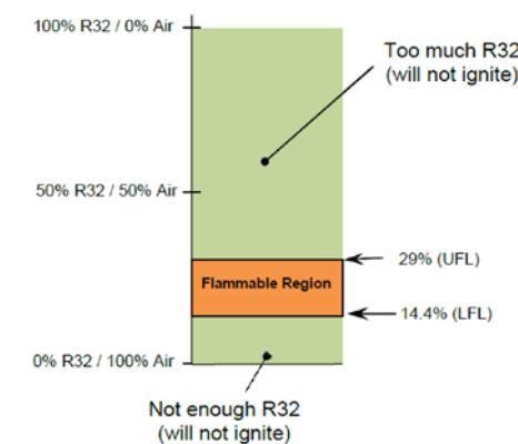
R32 lower flammability limit
