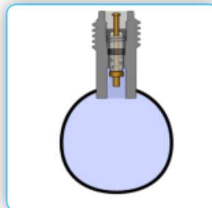
Cutaway showing plunger in valve stem
